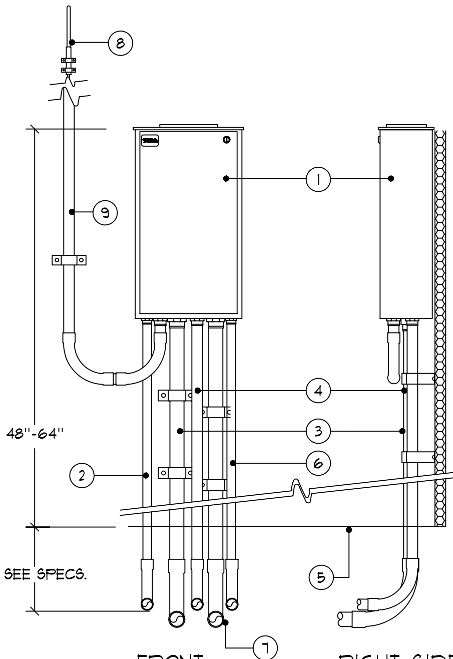
FRONT SECTION/ELEVATION RIGHT-SIDE SECTION/ELEVATION
